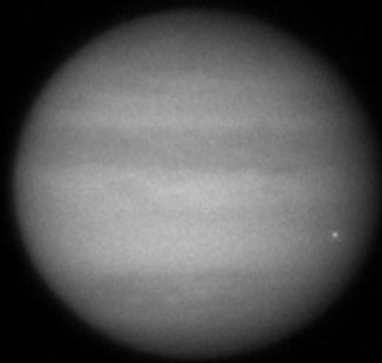
Jupiter impact June 3 20:31:29.15 Anthony Wesley, Broken Hill Australia
